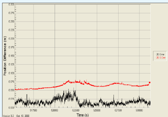
Figure 4: SMART-V1 Typical RT-20 Steady State (Horizontal)
