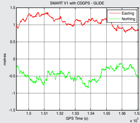
Figure 7: SMART-V1 (CDGPS): Least squares (left) and GL1DE (right)
