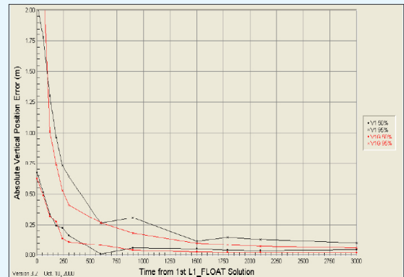
Figure 3: SMART-V1 and SMART-V1G – Vertical Convergence of RT-20 Solution
