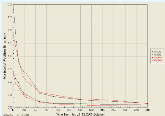
Figure 2: SMART-V1 and SMART-V1G – Horizontal Convergence of RT-20 Solution
